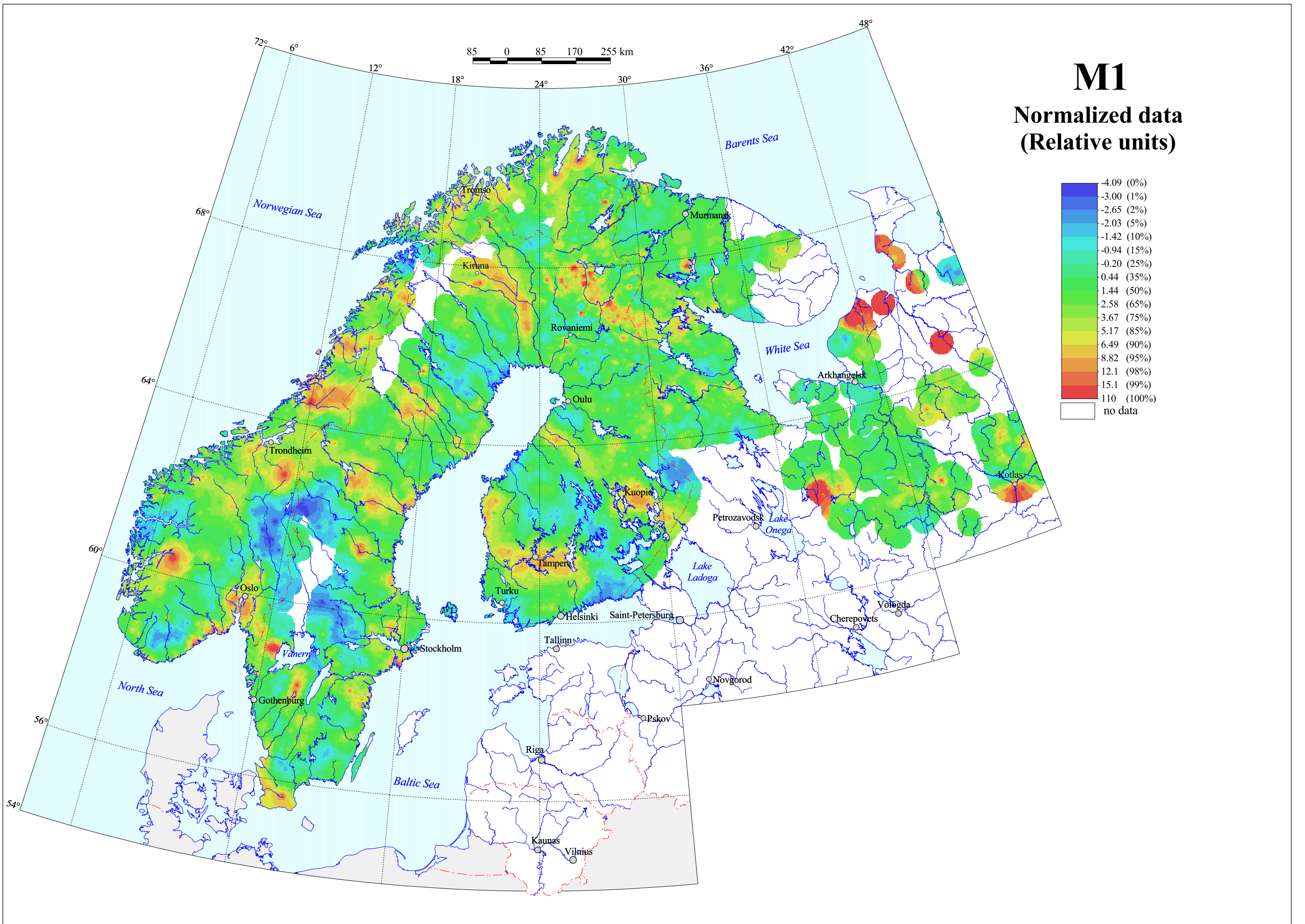
M1 (Co, Cr, Cu, Mg, Ni, V) in Till, Grain Size <0.06 mm
